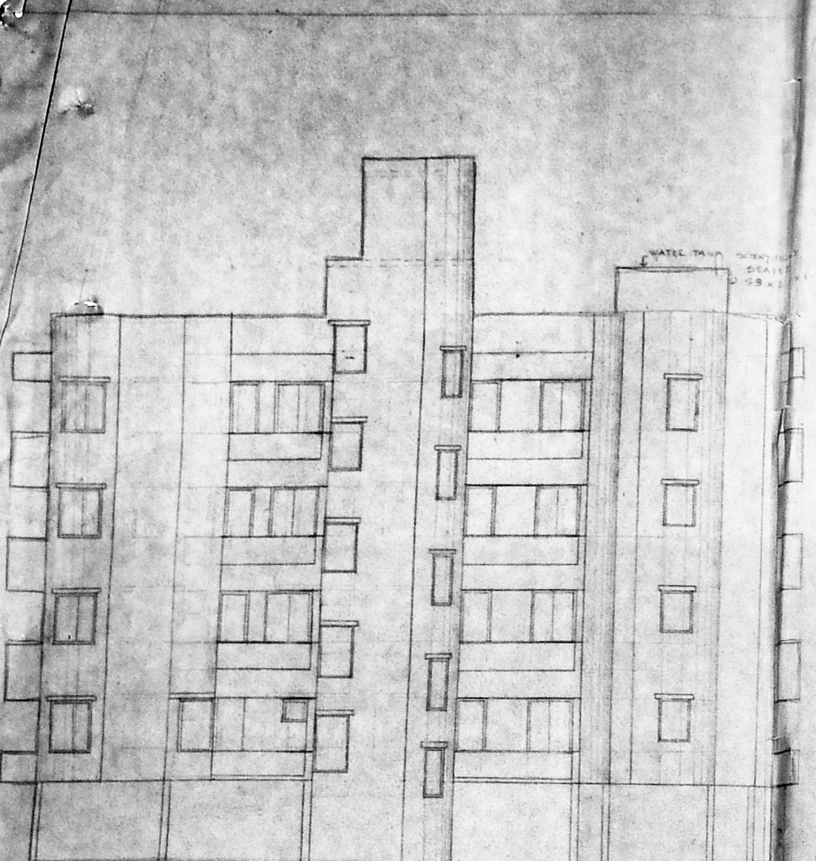
FRONT ELEVATION
